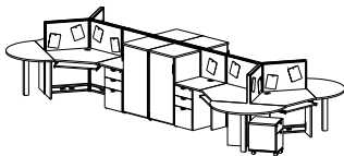
13. 120° radial dogbone featuring 388 series
